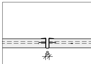
FUGENPROFIL JOINT PROFILE JOINT PROFILE
