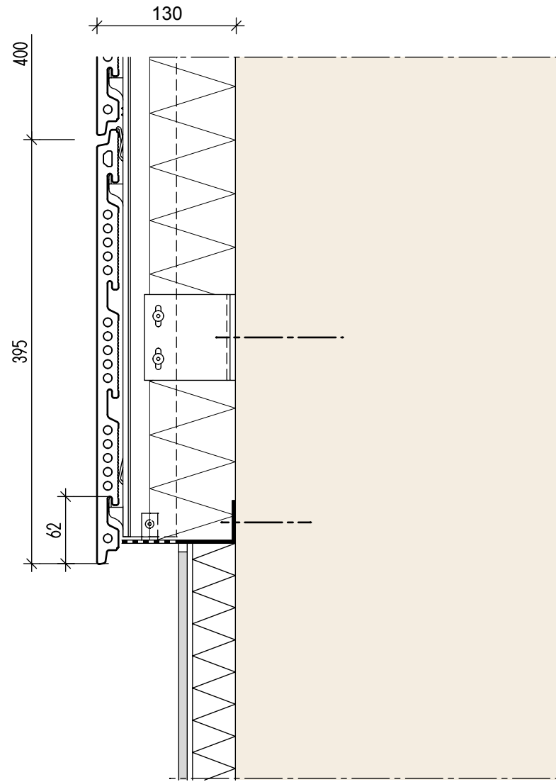
CONNECTION TO PLINTH SC. 1:5
