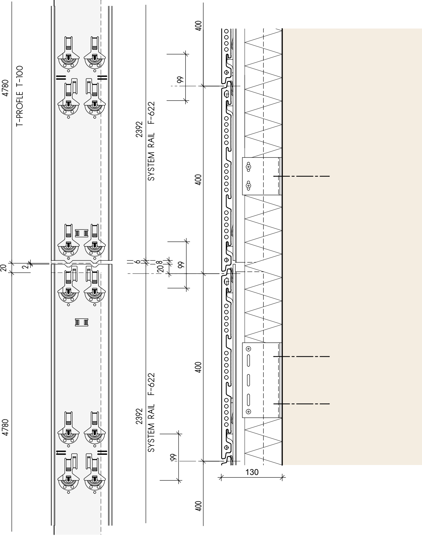
BUTT-JOINT OF PROFILES SC. 1:5 DETAIL "D"
