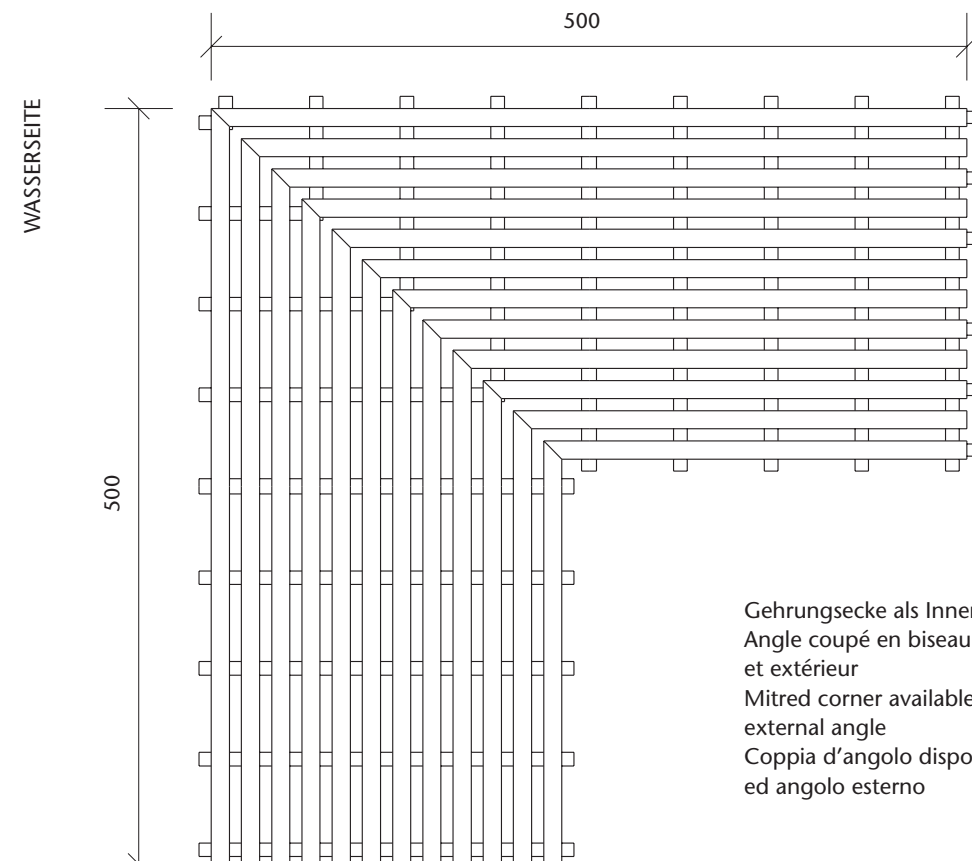
Parallelrost/Grille parallèle/Parallel grating/Griglia parallela
